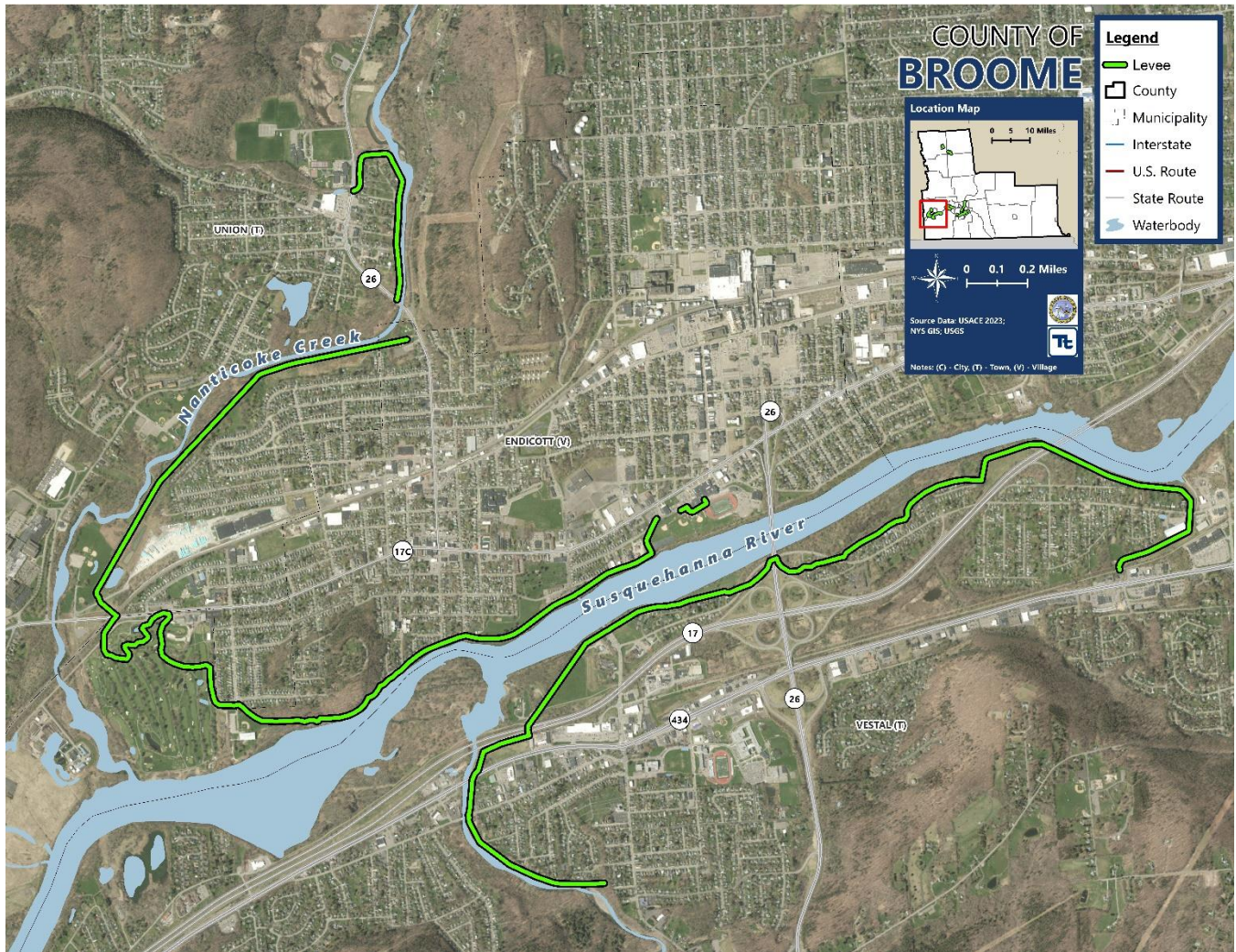
Figure 3-17. Endicott-Vestal-Union Levee
